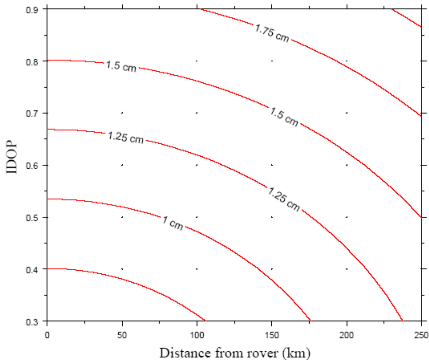
OPUS-RS expected horizontal standard error (cm) as a function of distance from rover and IDOP (15 minutes observation span)
